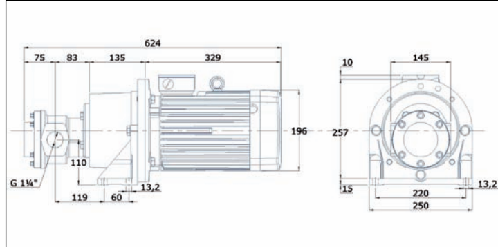
FOM 545- FOM 556 4,0 kW weight: 40 kg
