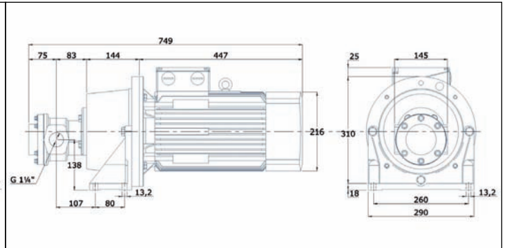
FOM 545- FOM 556 11 kW weight: 82 kg
