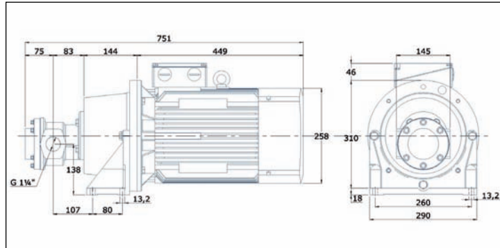
FOM 545- FOM 556 15 kW weight: 116 kg
