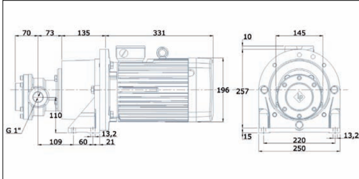
FOM 422- FOM 438 4,0 kW weight: 38,5 kg
