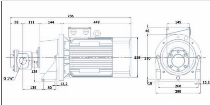
FOM 570- FOM 590 15 kW weight: 119 kg
