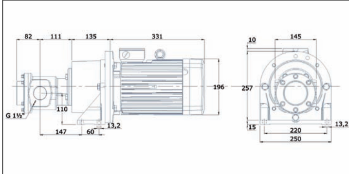
FOM 570- FOM 590 4,0 kW weight: 43 kg
