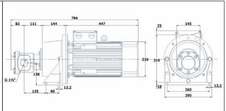
FOM 570- FOM 590 11 kW weight: 85 kg
