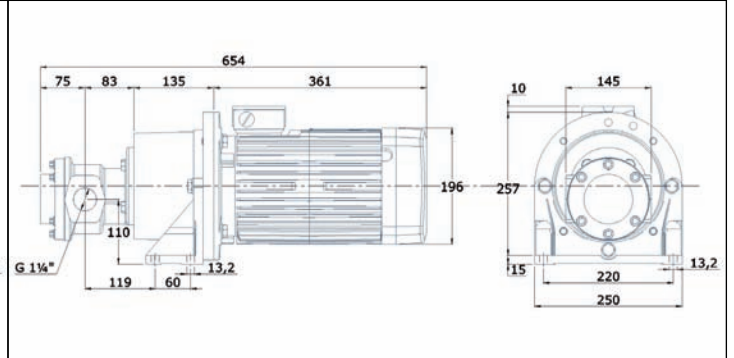
FOM 545- FOM 556 5,5 kW weight: 57 kg
